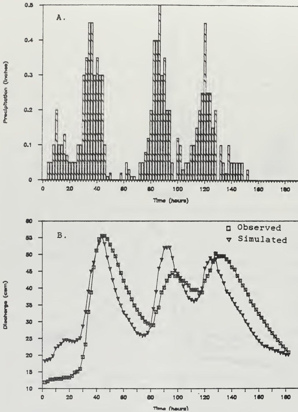
Figure 30. (A) Hyetograph, and (B) simulated and observed hydrographs for a "complex" rainfall event on Flynn Creek, Oregon Coast Range (January 5-13, 1969). The API method closely simulates the shape of a hydrograph resulting from a complex rainfall event.
